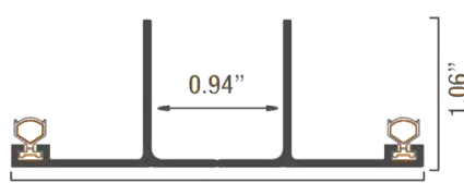
Lower Aluminum Profile 16/25
