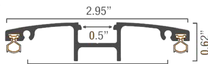
Upper Aluminum Profile
