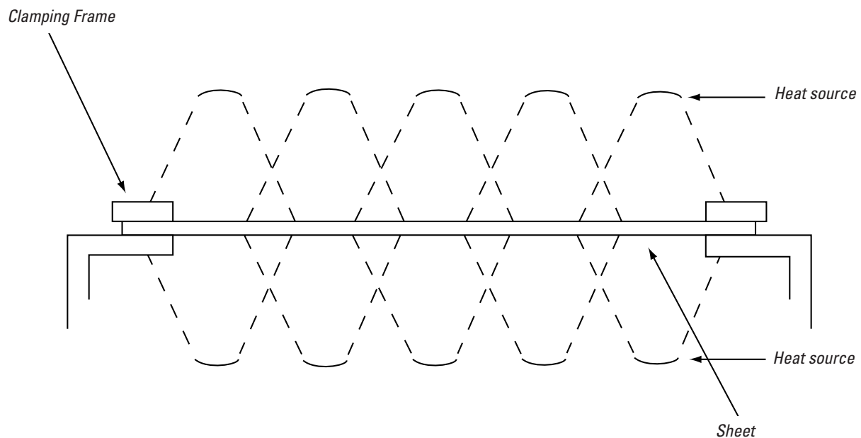
Fig. 1.5: Sandwich Heating
