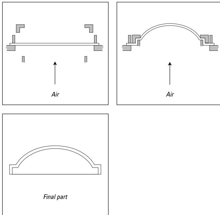
Fig. 1.16: Free-blown Domes
